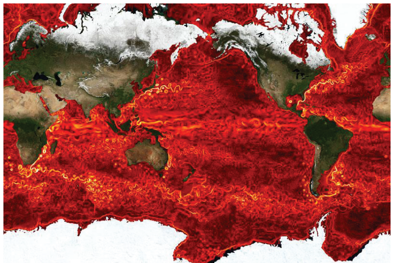
Surface current speeds from a 1/16-degree solution simulation. Image: Chris Henze, NASA/Ames
