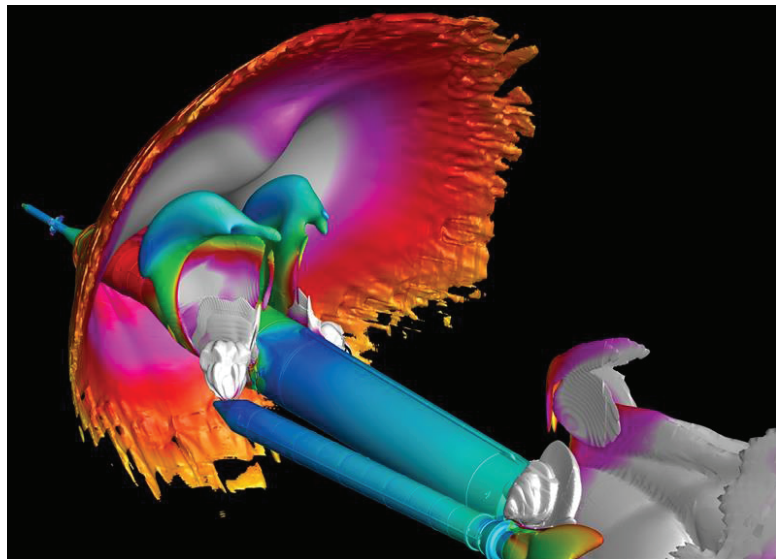
Space Launch System (SL S) booster separation flow field. Stuart Rogers, NASA/Ames
